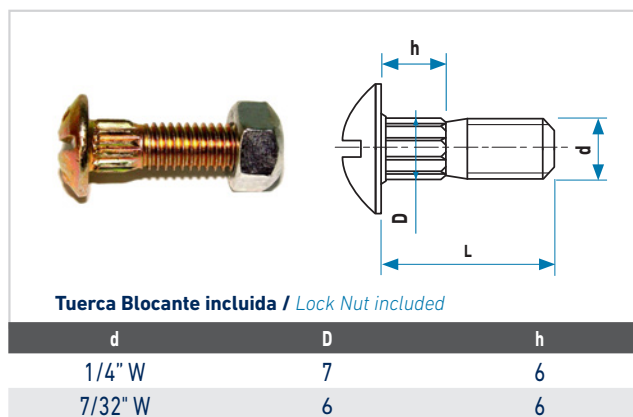
Moleteado cab. Redonda / Knurled round head
